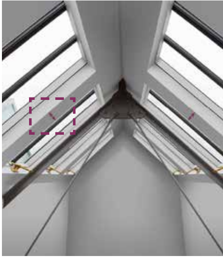
Option 1. Linking Bars (Linking standard roof windows) 310mm between viewables.
